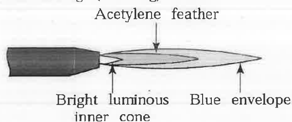
(c) Carburizing (reducing) flame
