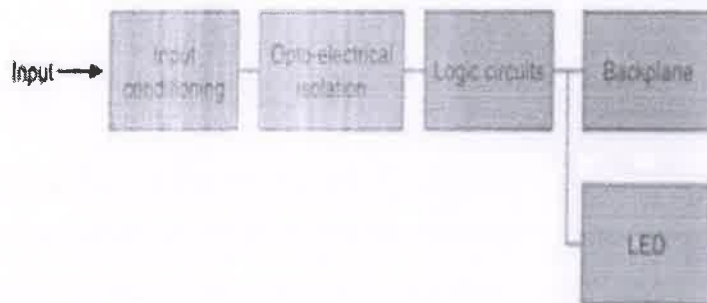
Block diagrams of a discrete input module.
