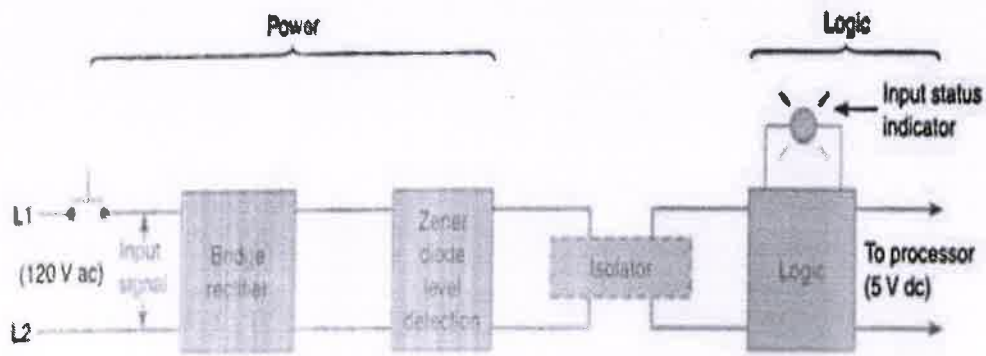
Block diagrams of a discrete input module.
