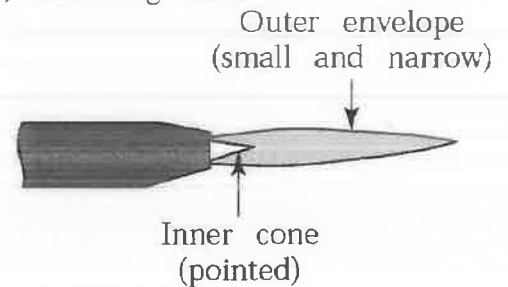
(b) Oxidizing flame
